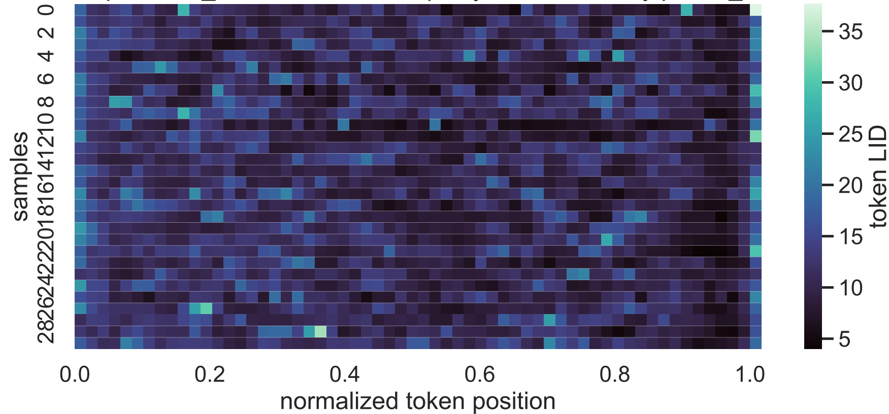
4B Exp C think_answer LID heatmap, layer 20, sorted by paired_delta
