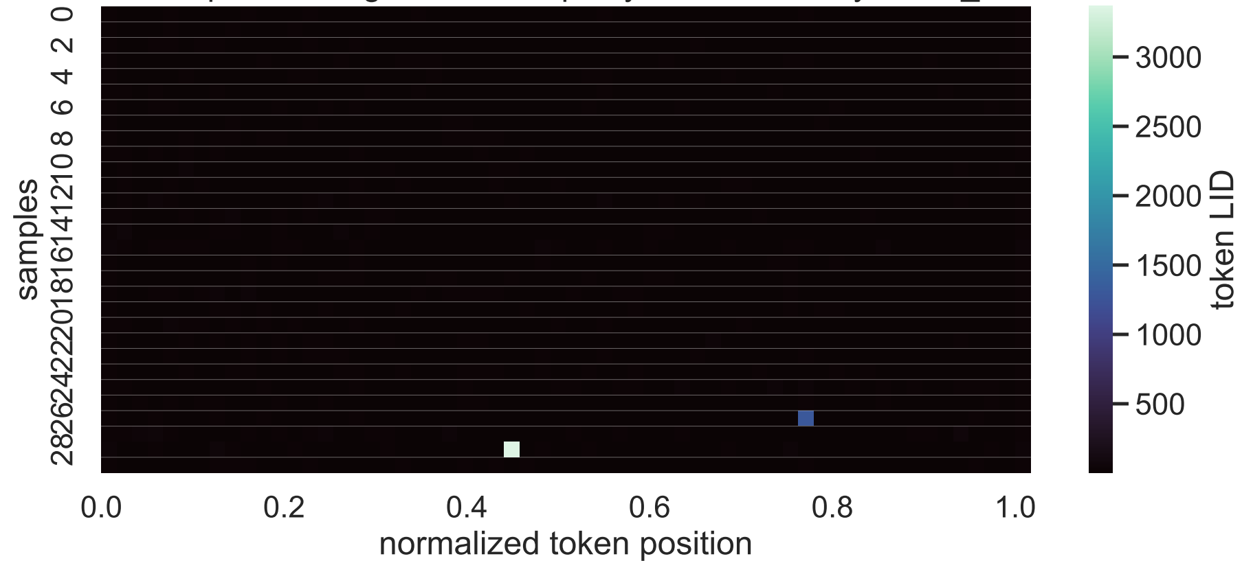
4B Exp C thinking LID heatmap, layer 20, sorted by mean_lid
