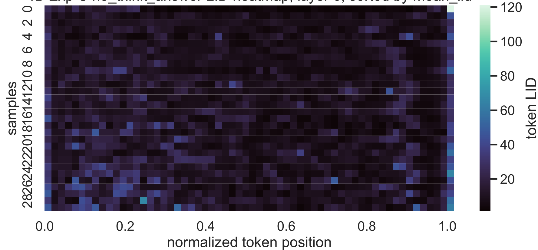
4B Exp C no_think_answer LID heatmap, layer 6, sorted by mean_lid
