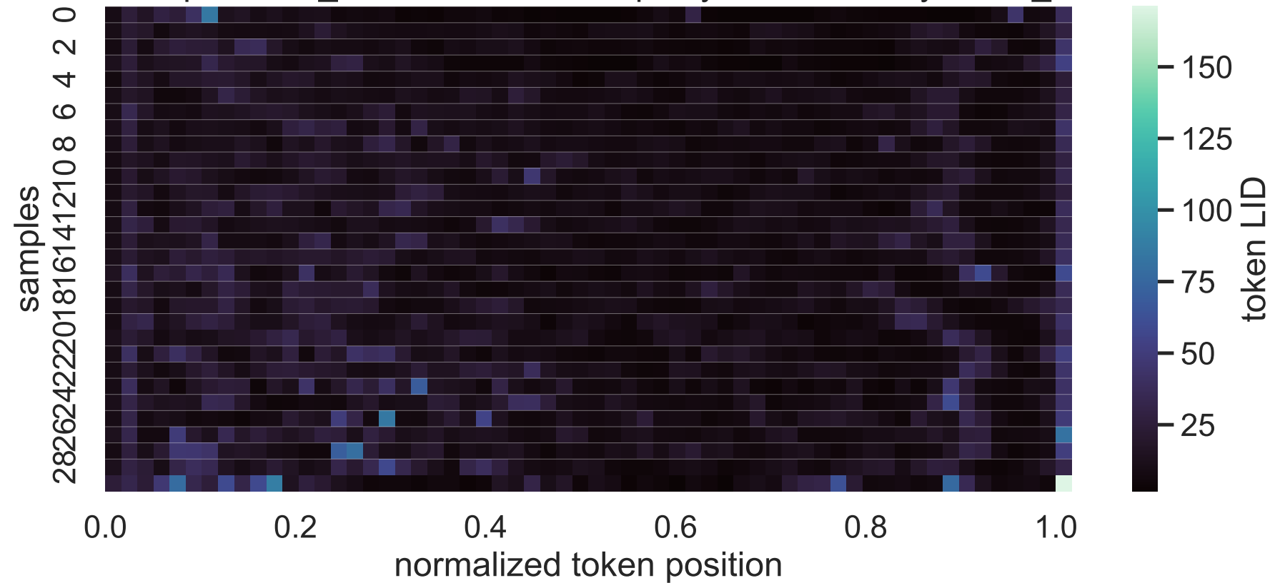
4B Exp C think_answer LID heatmap, layer 6, sorted by mean_lid
