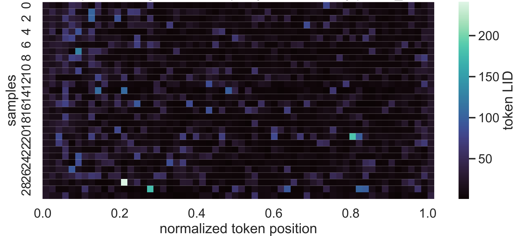
4B Exp C thinking LID heatmap, layer 6, sorted by paired_delta
