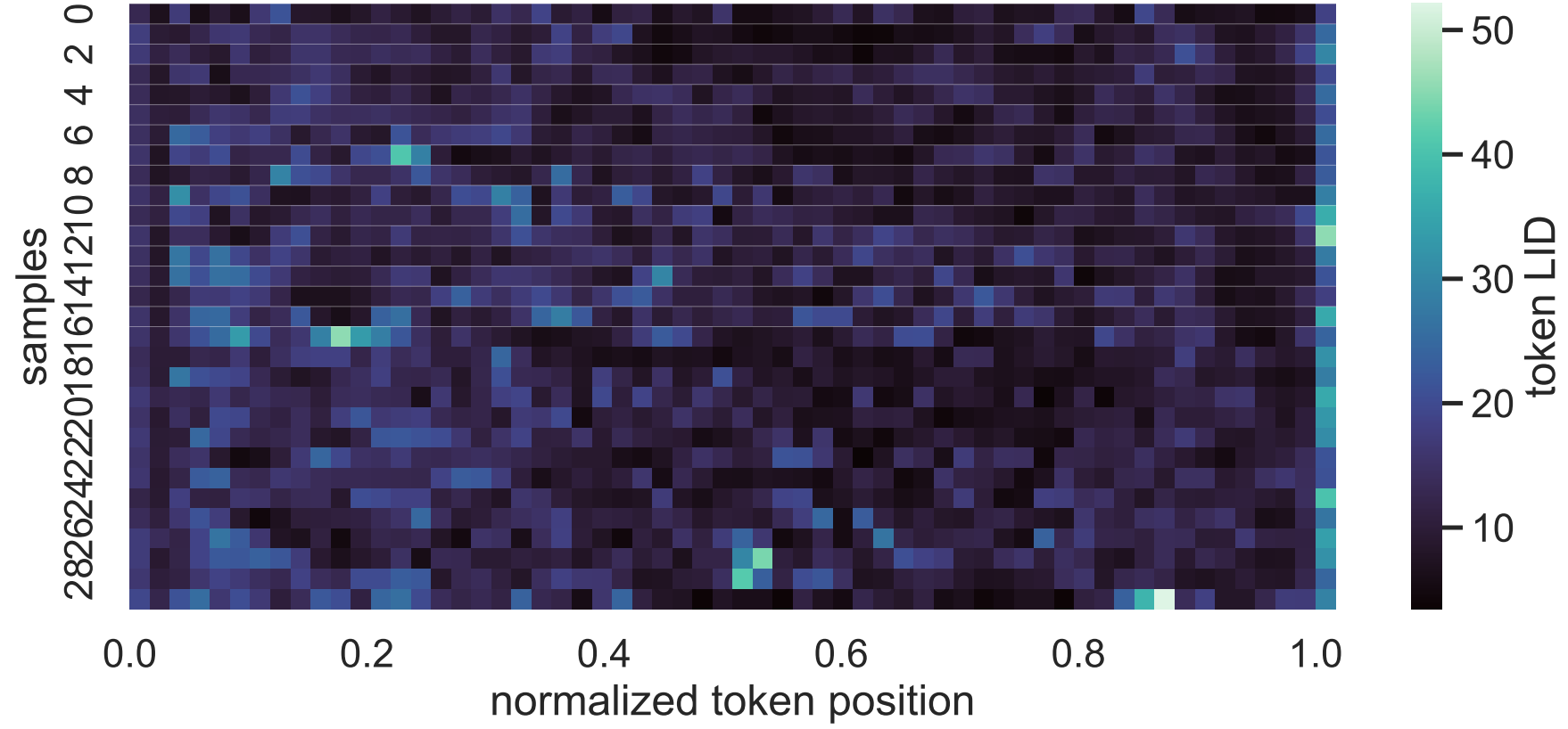
8B Exp C no_think_answer LID heatmap, layer 13, sorted by correctness_then_mean_lid
