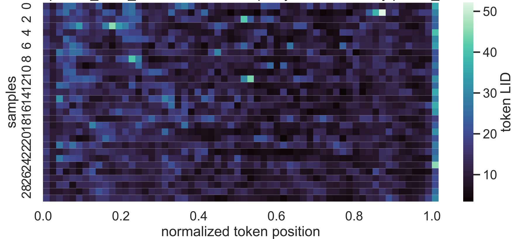
8B Exp C no_think_answer LID heatmap, layer 13, sorted by paired_delta
