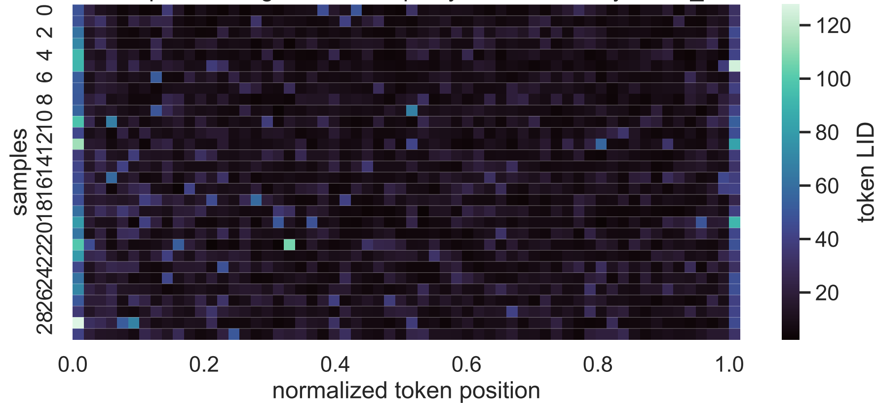
8B Exp C thinking LID heatmap, layer 13, sorted by mean_lid
