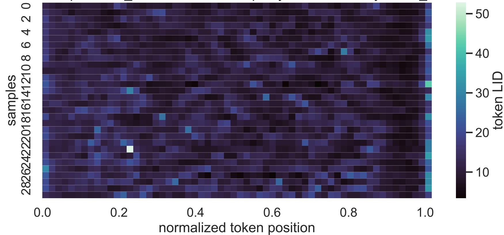
8B Exp C think_answer LID heatmap, layer 20, sorted by mean_lid
