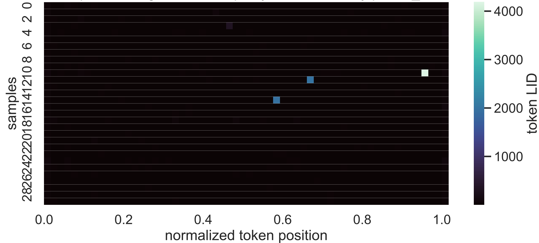
8B Exp C thinking LID heatmap, layer 20, sorted by paired_delta
