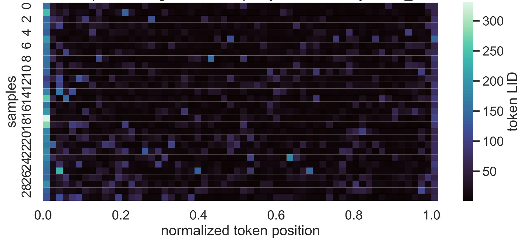
8B Exp C thinking LID heatmap, layer 6, sorted by mean_lid
