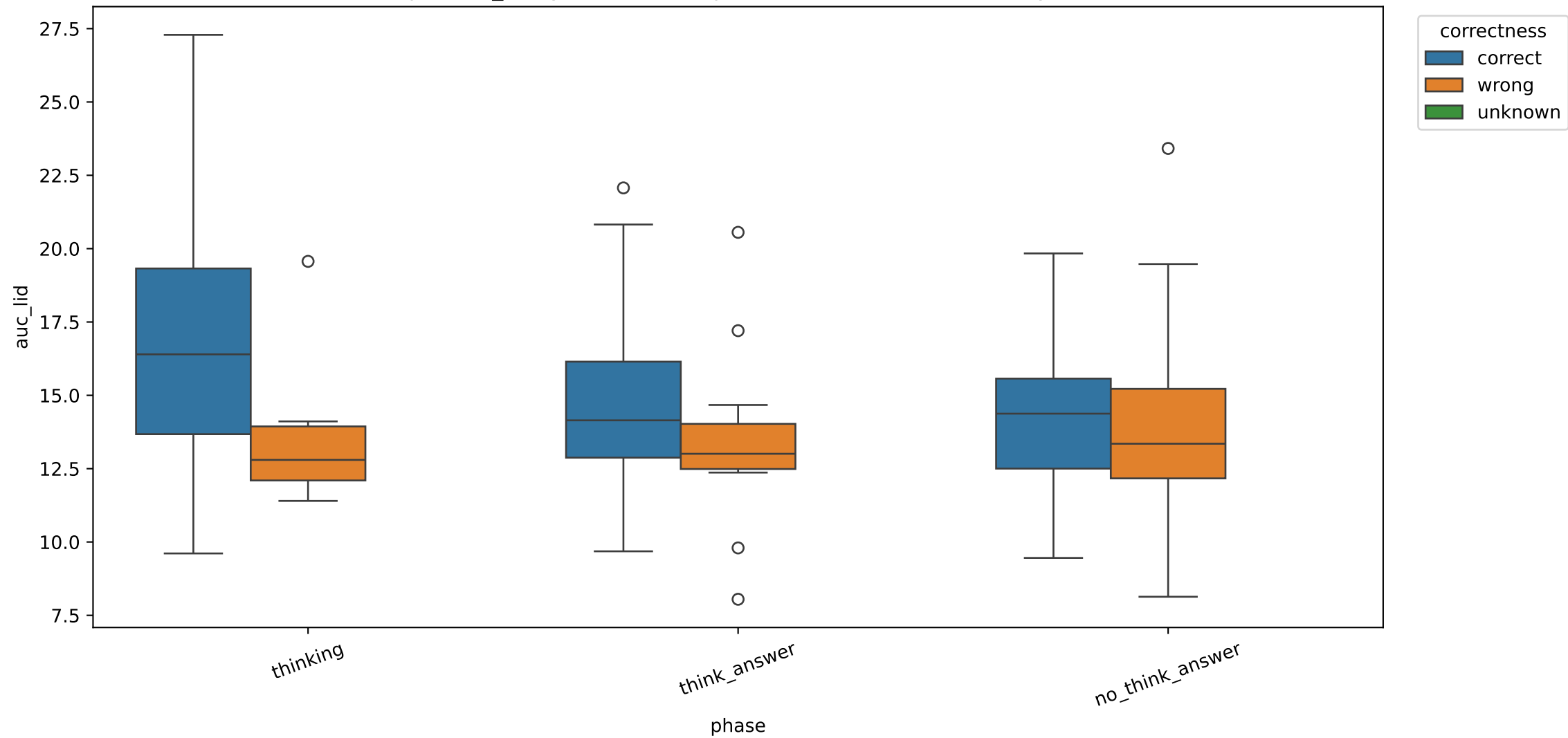
Exp C auc_lid by correctness, pooled across model sizes, layer 6
