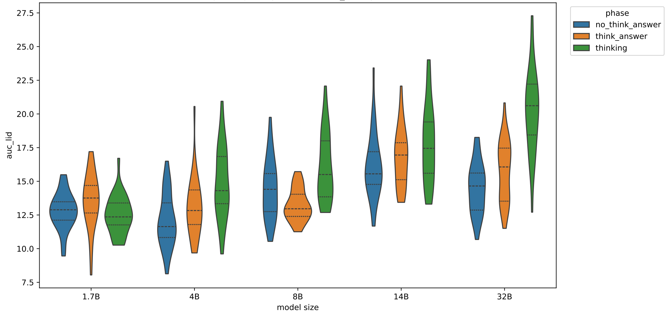
Exp C trajectory statistic: auc_lid, layer 6
