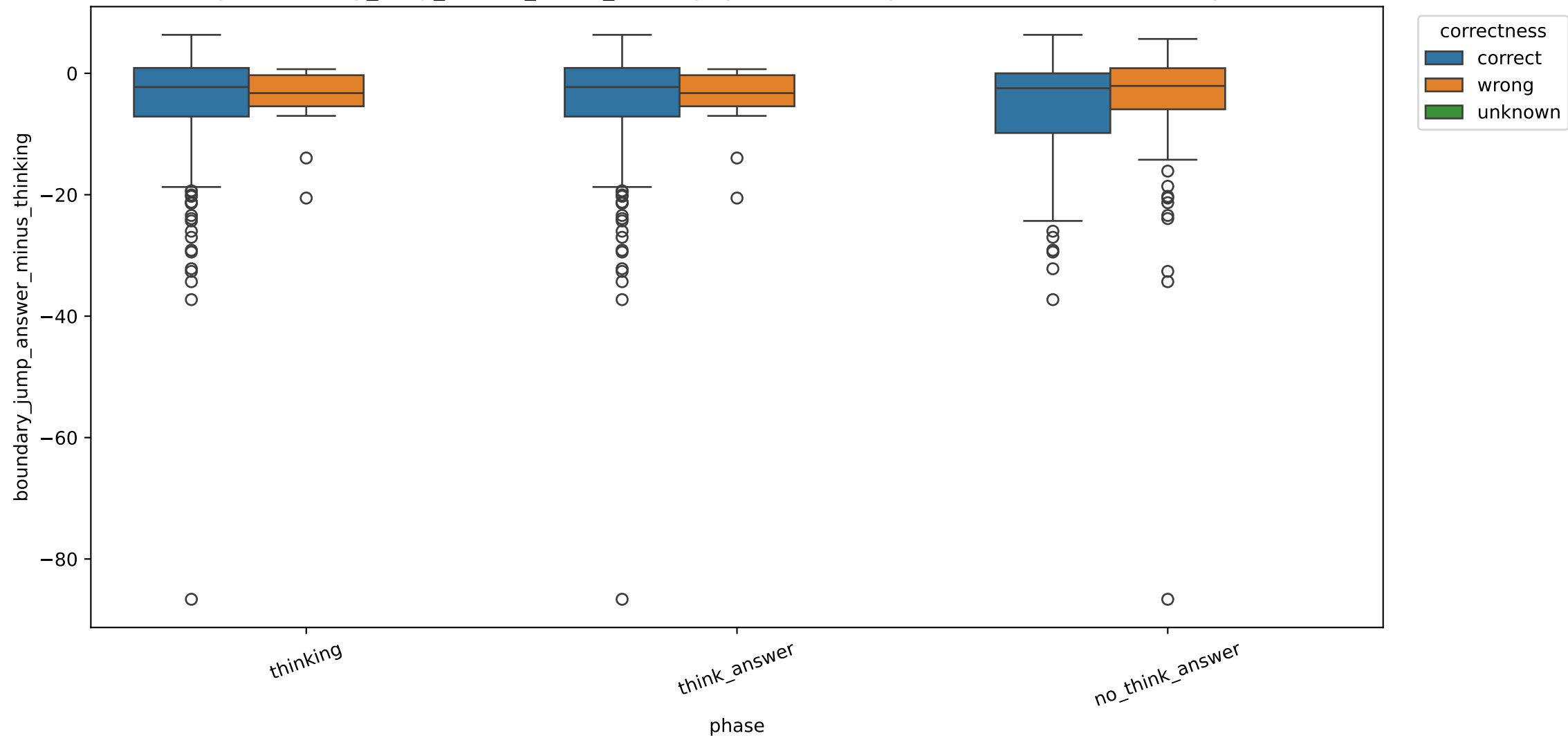
Exp C boundary_jump_answer_minus_thinking by correctness, pooled across model sizes, layer 20
