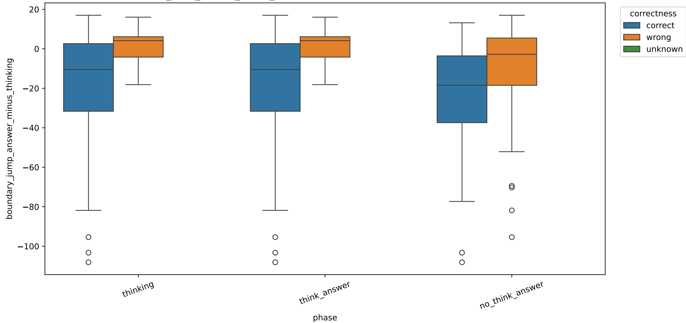
Exp C boundary_jump_answer_minus_thinking by correctness, pooled across model sizes, layer 6
