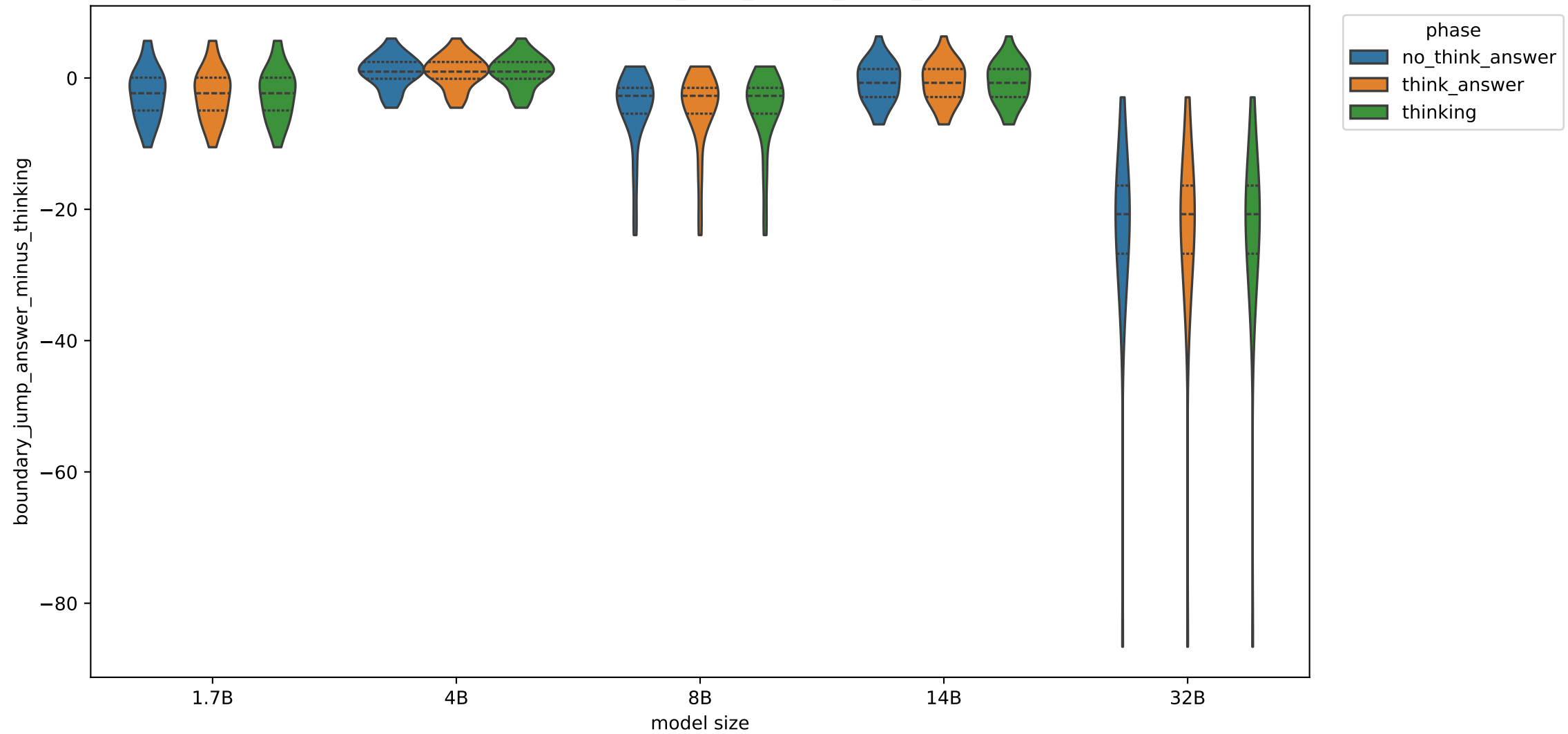
Exp C trajectory statistic: boundary_jump_answer_minus_thinking, layer 20
