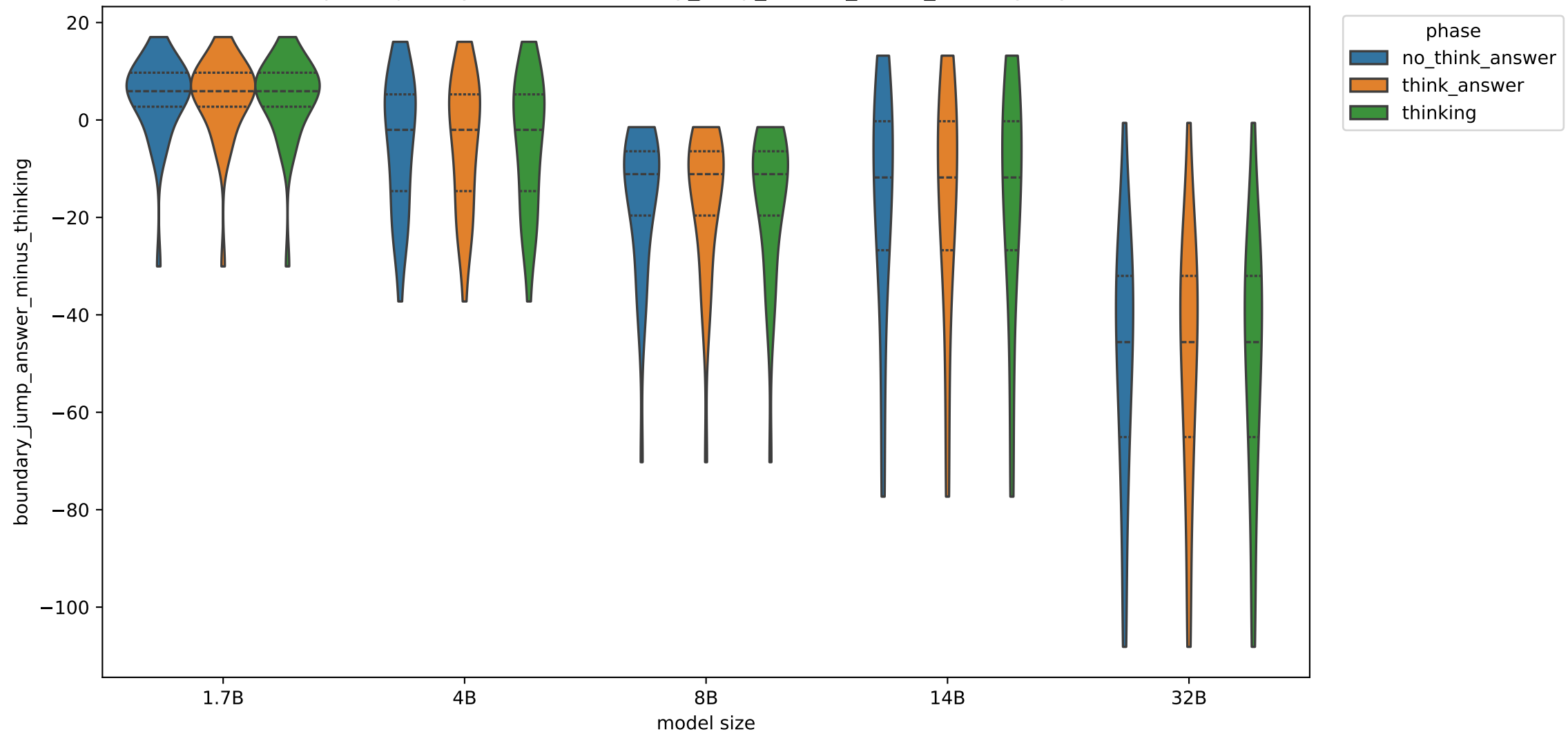
Exp C trajectory statistic: boundary_jump_answer_minus_thinking, layer 6
