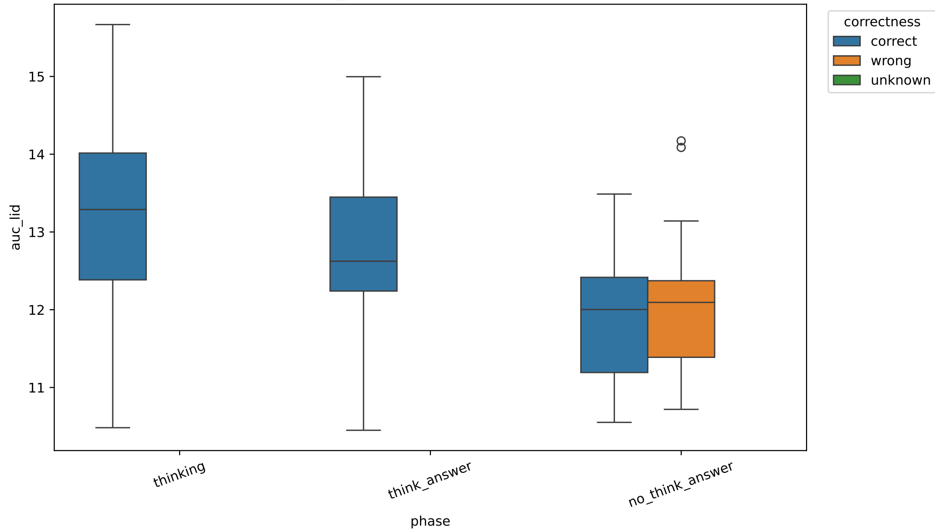
Exp C auc_lid by correctness, 14B, layer 13
