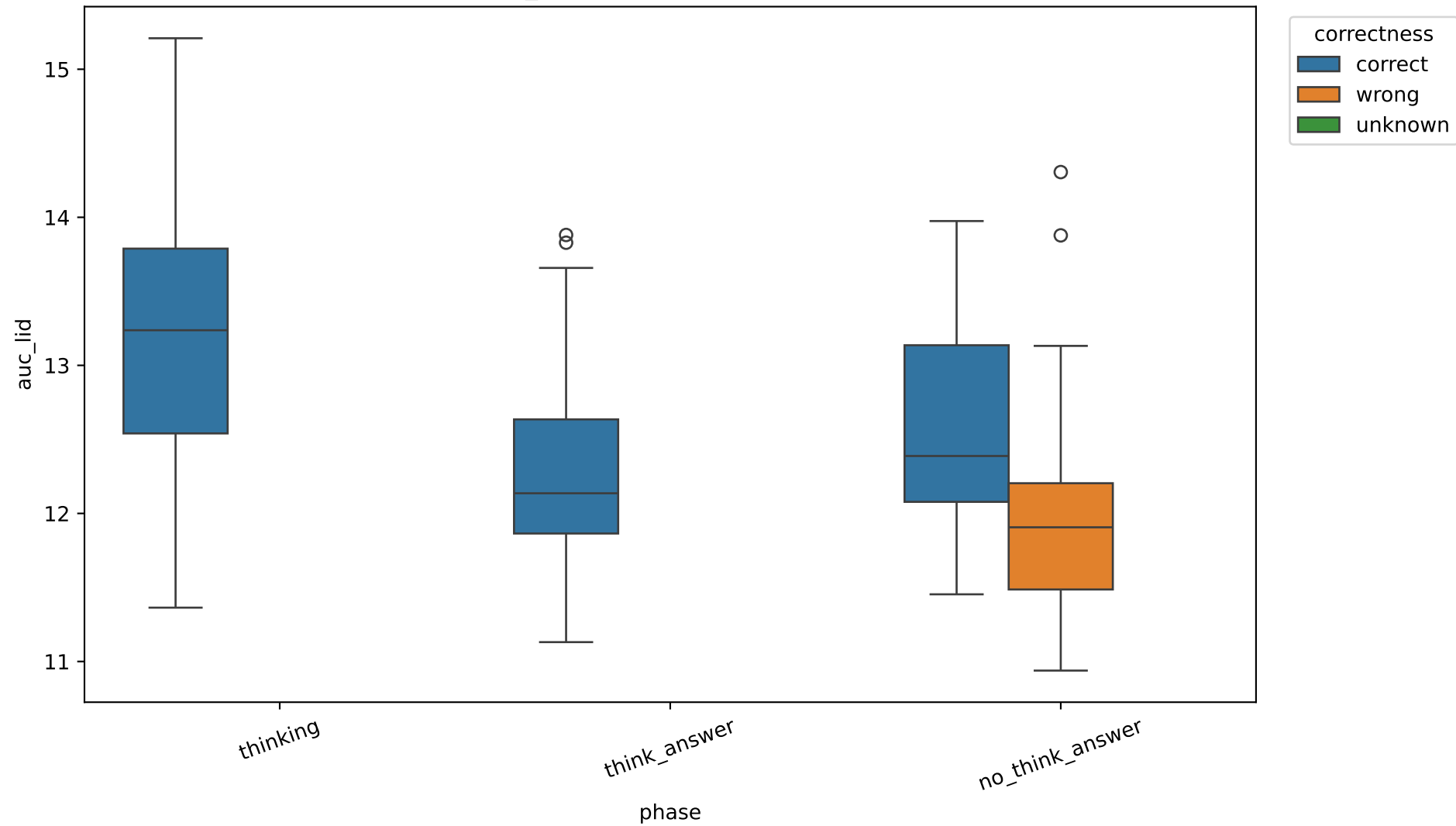
Exp C auc_lid by correctness, 14B, layer 20
