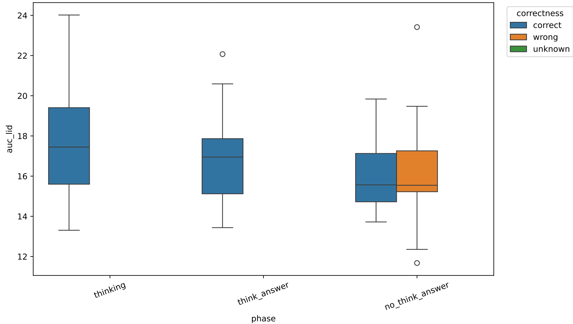
Exp C auc_lid by correctness, 14B, layer 6
