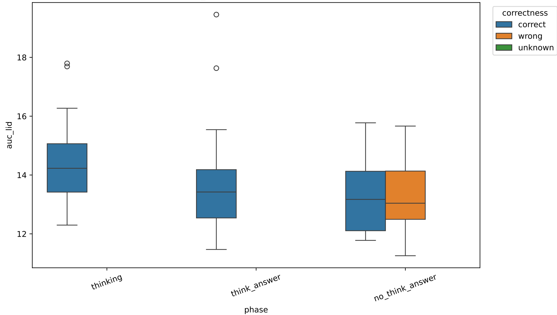
Exp C auc_lid by correctness, 32B, layer 13
