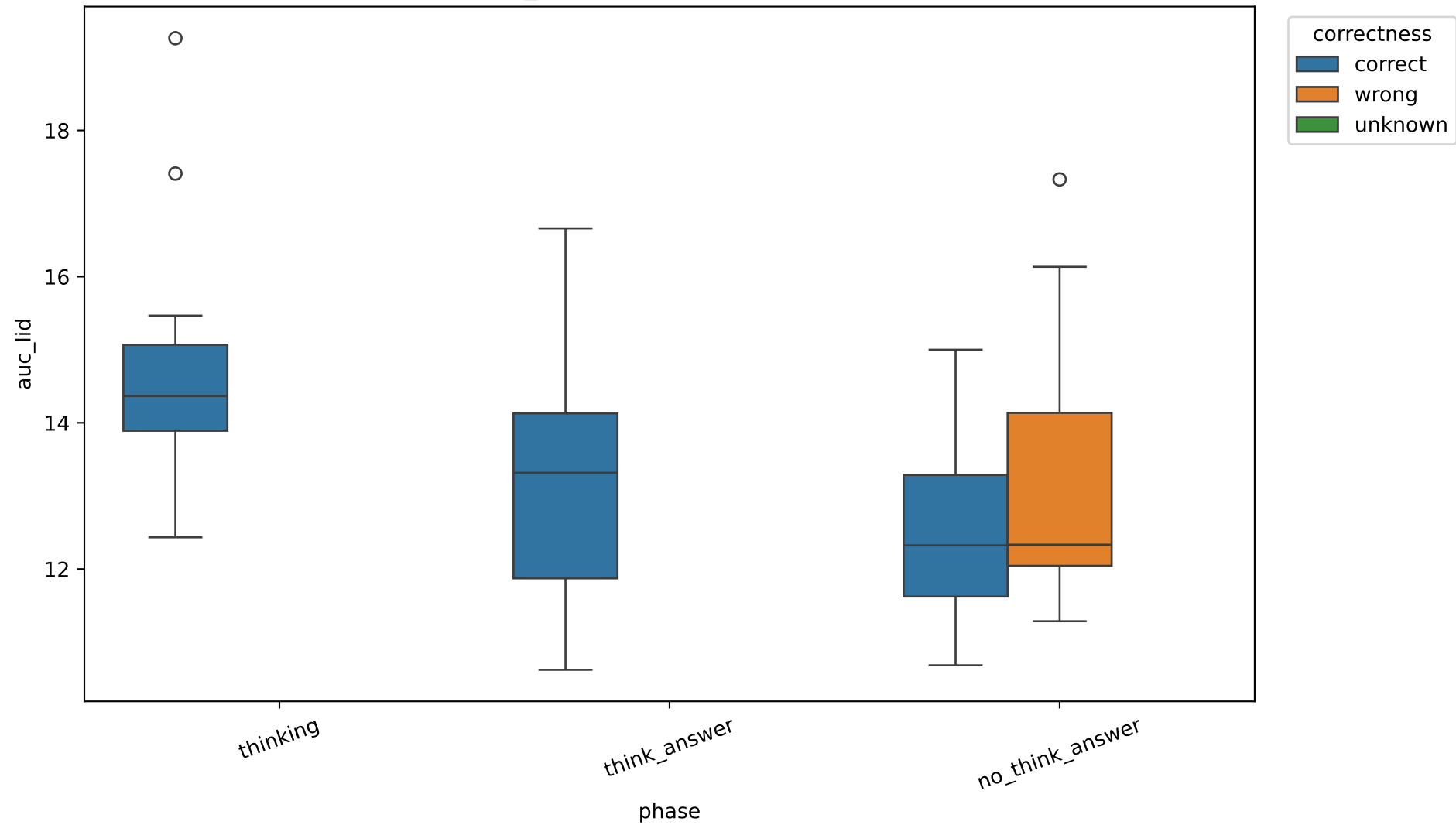
Exp C auc_lid by correctness, 32B, layer 20
