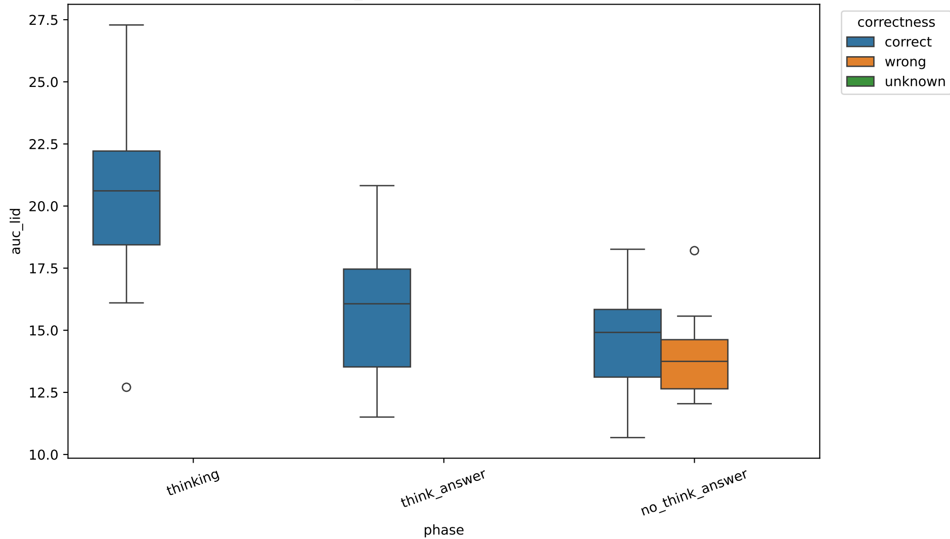
Exp C auc_lid by correctness, 32B, layer 6
