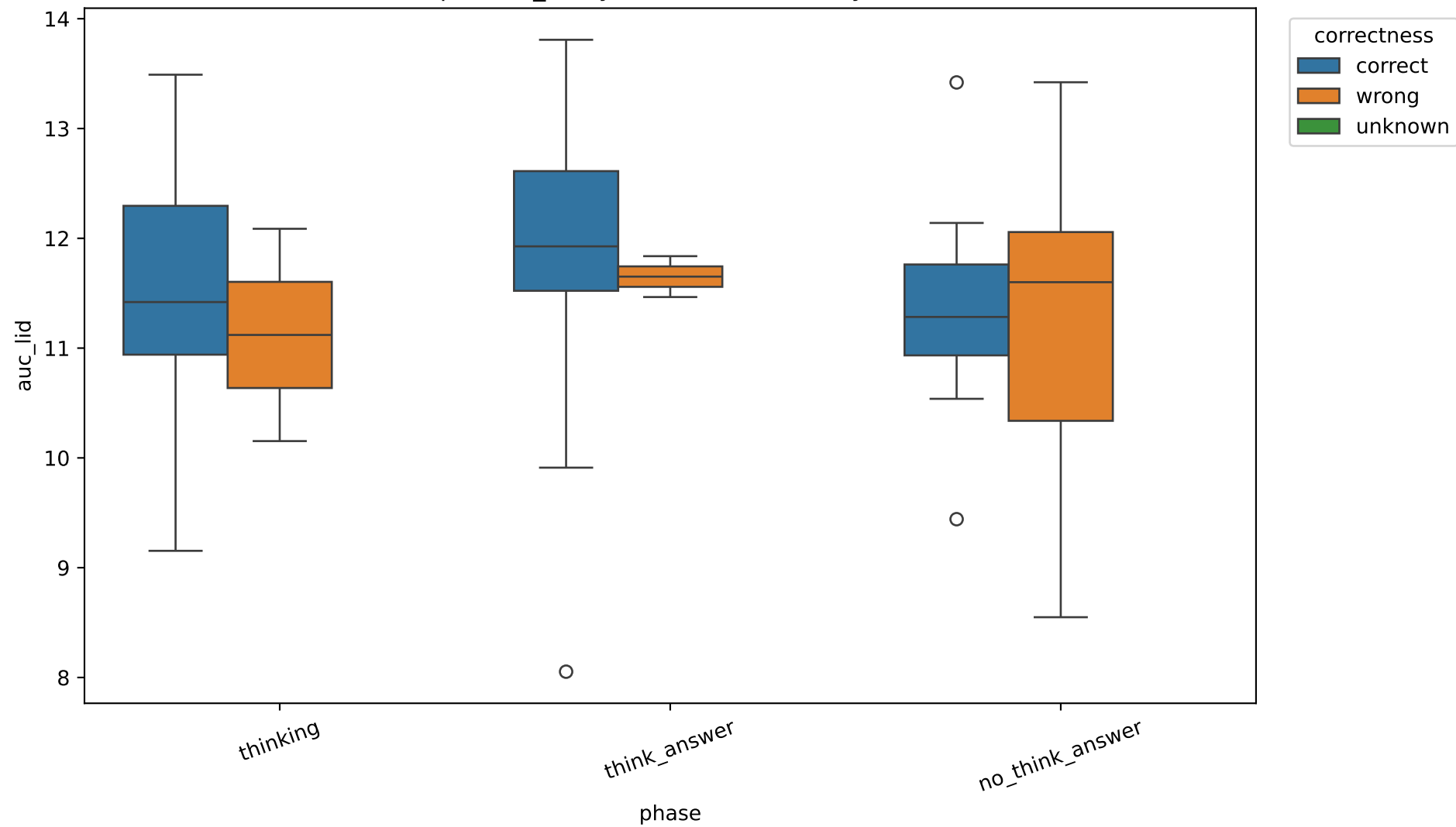
Exp C auc_lid by correctness, 4B, layer 13
