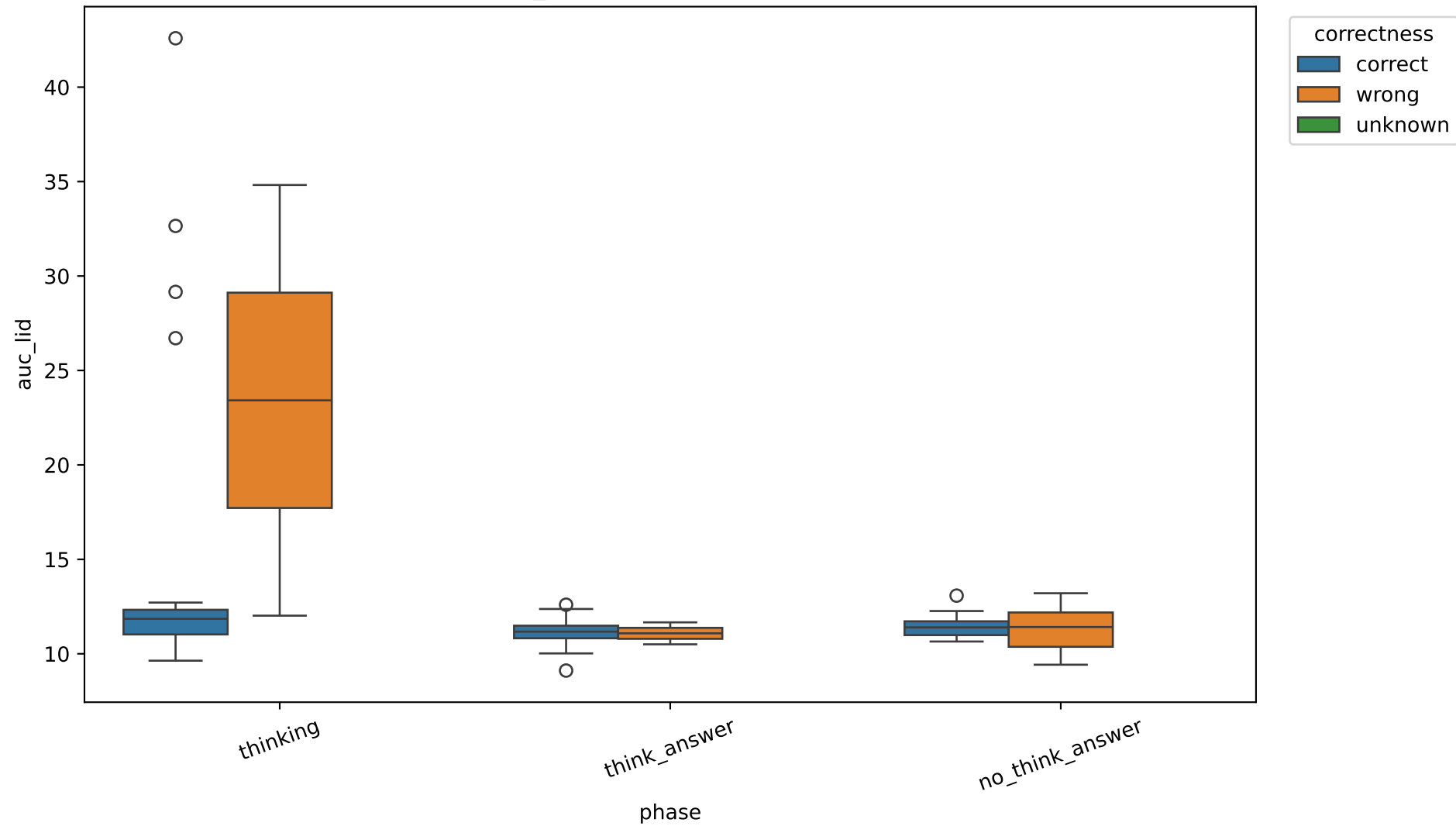
Exp C auc_lid by correctness, 4B, layer 20
