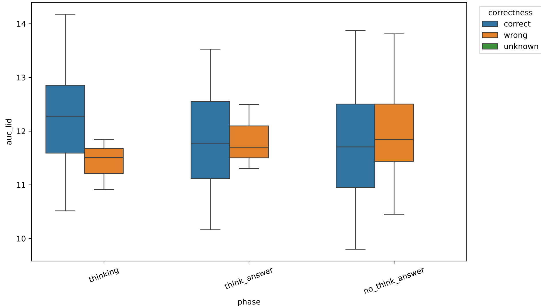
Exp C auc_lid by correctness, 8B, layer 13
