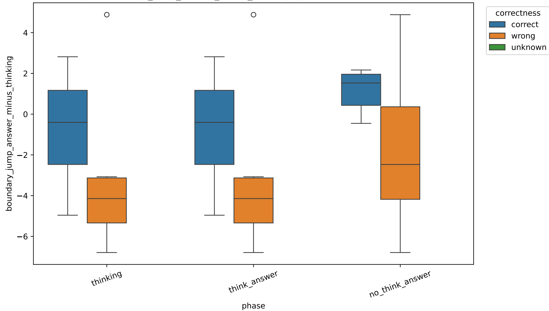
Exp C boundary_jump_answer_minus_thinking by correctness, 1.7B, layer 13
