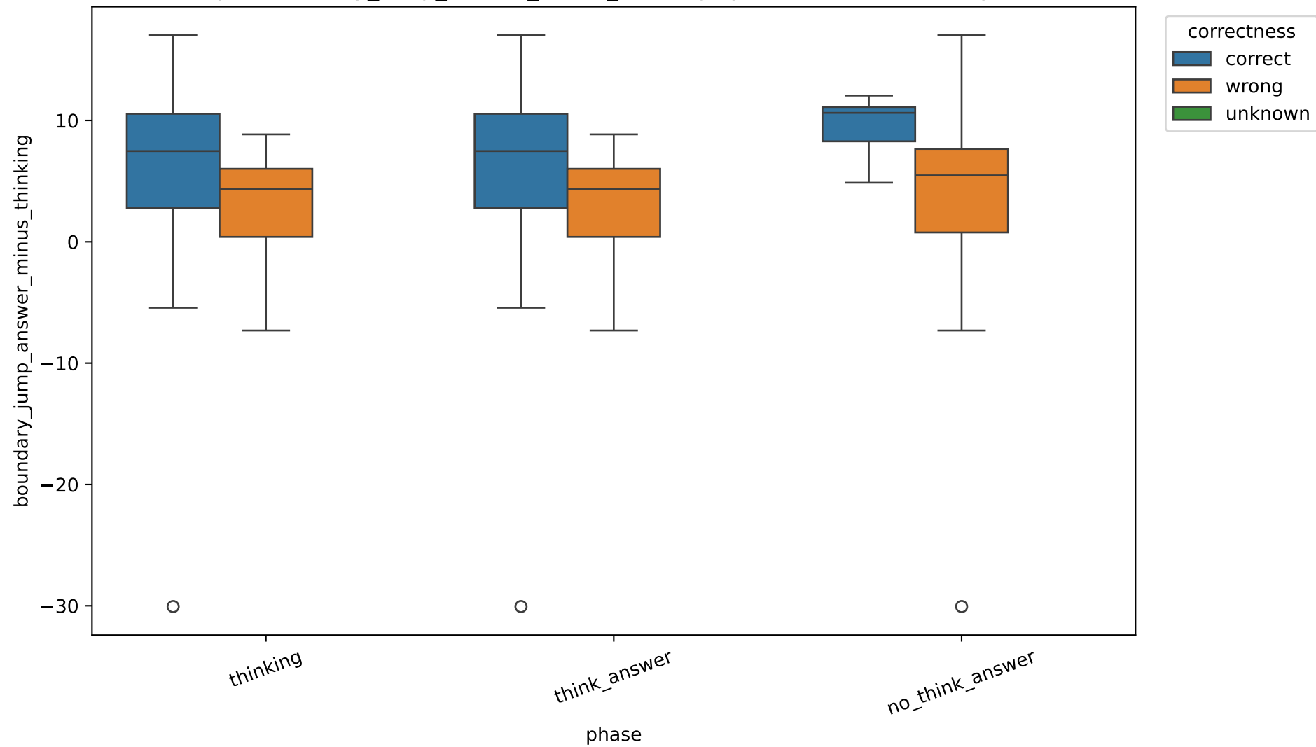
Exp C boundary_jump_answer_minus_thinking by correctness, 1.7B, layer 6
