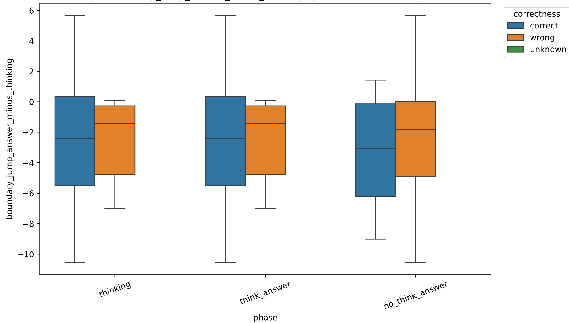
Exp C boundary_jump_answer_minus_thinking by correctness, 1.7B, layer 20
