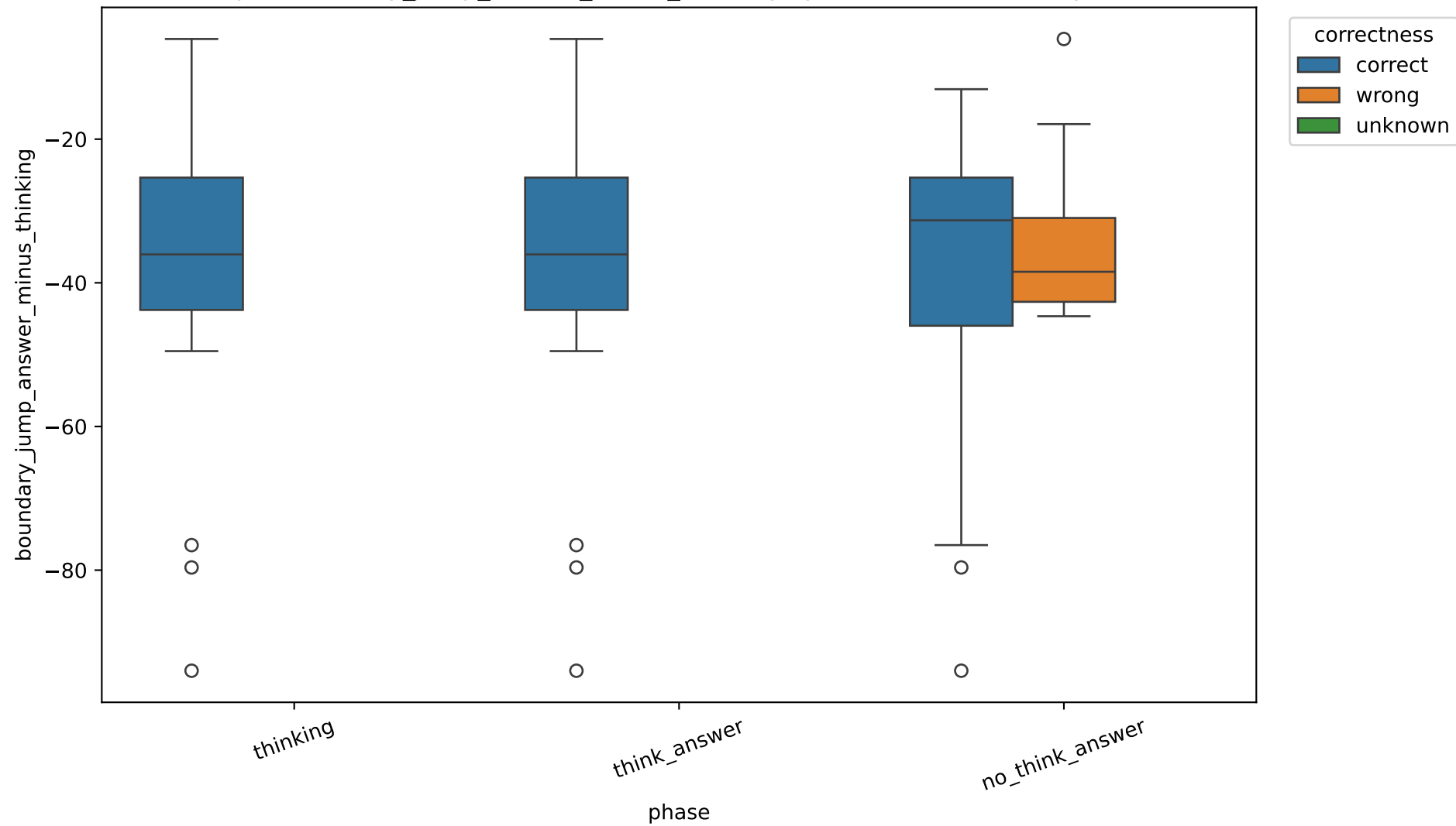
Exp C boundary_jump_answer_minus_thinking by correctness, 32B, layer 13
