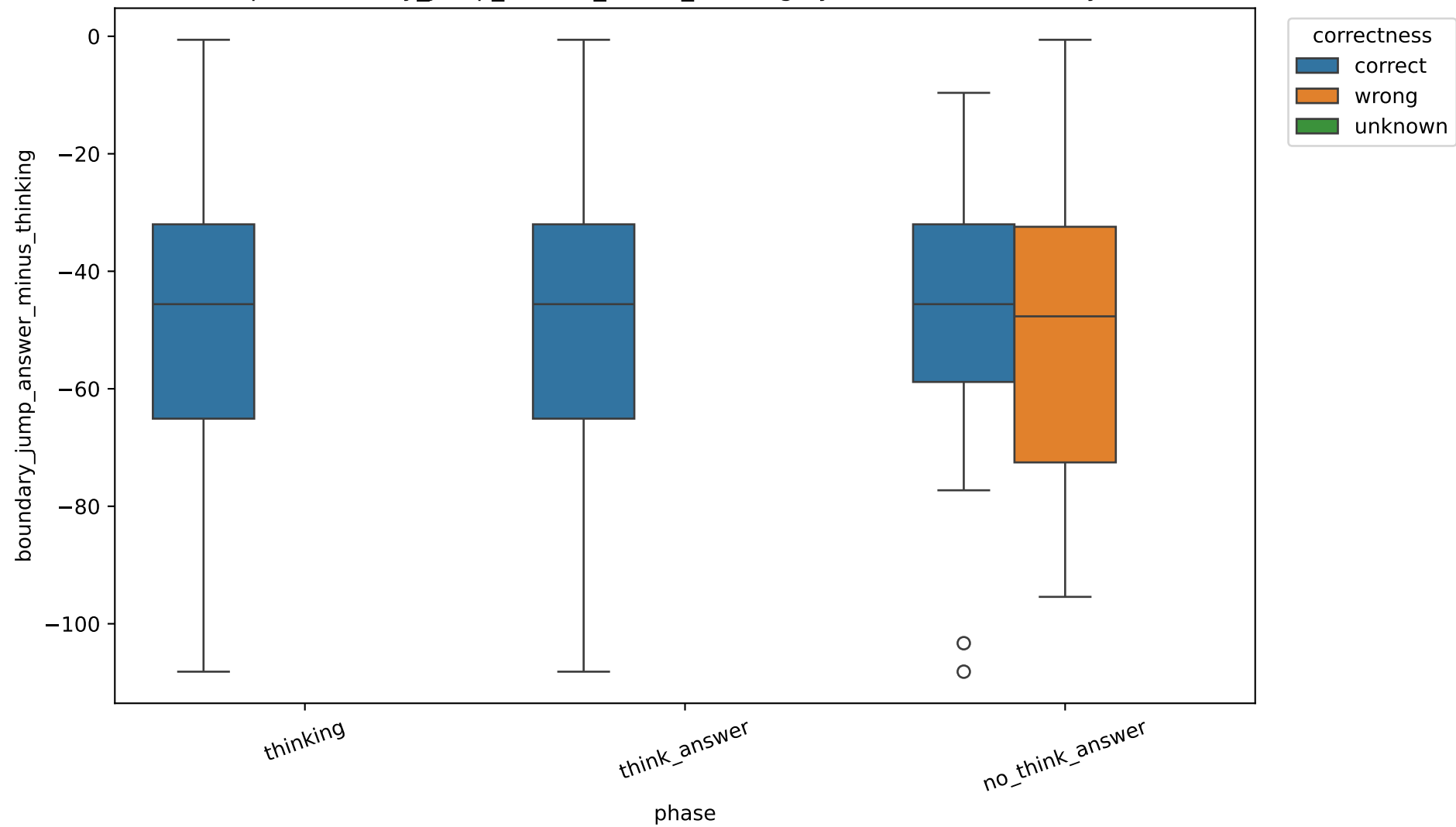
Exp C boundary_jump_answer_minus_thinking by correctness, 32B, layer 6
