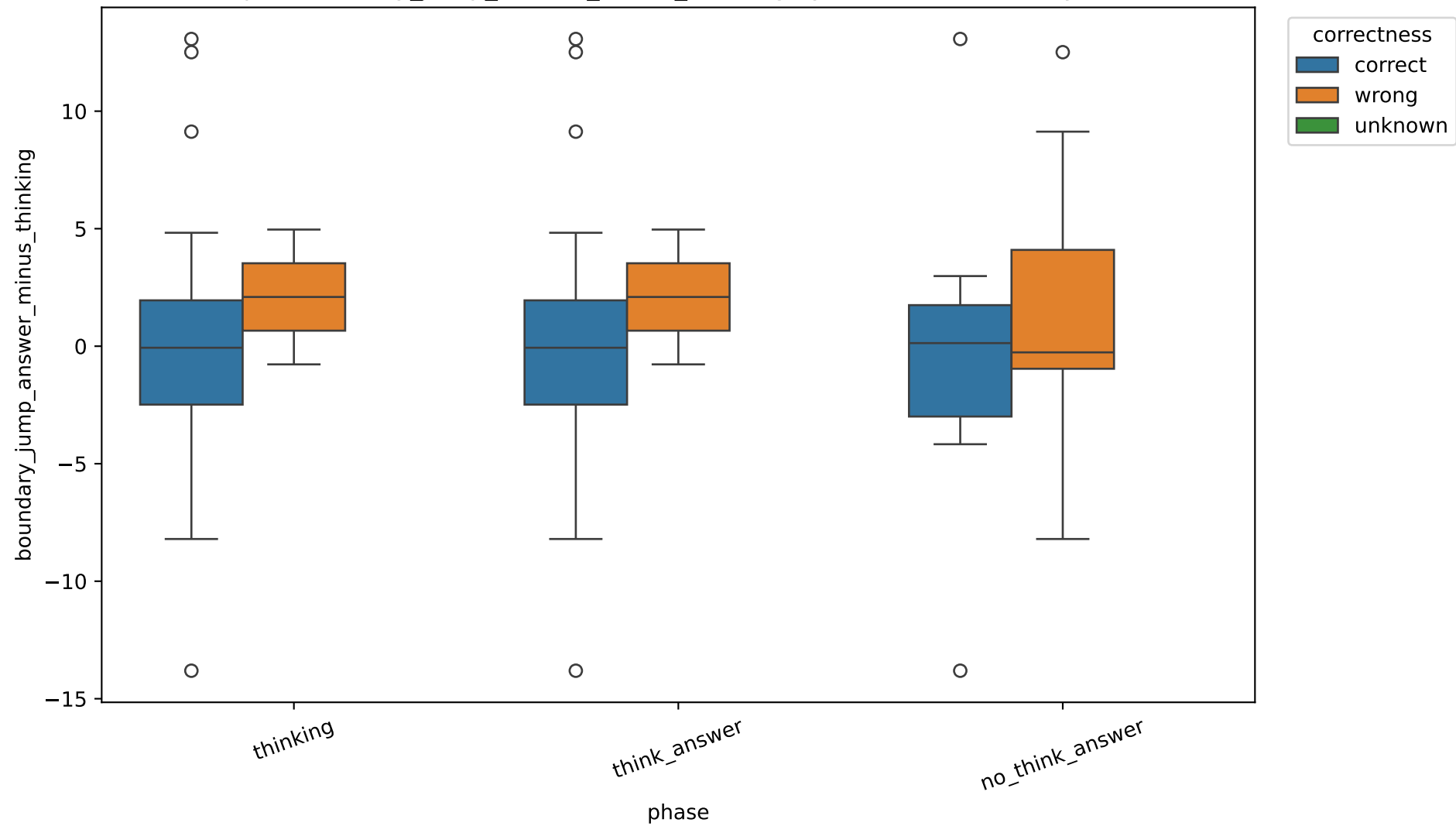
Exp C boundary_jump_answer_minus_thinking by correctness, 4B, layer 13
