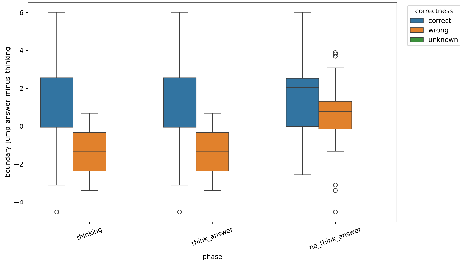
Exp C boundary_jump_answer_minus_thinking by correctness, 4B, layer 20
