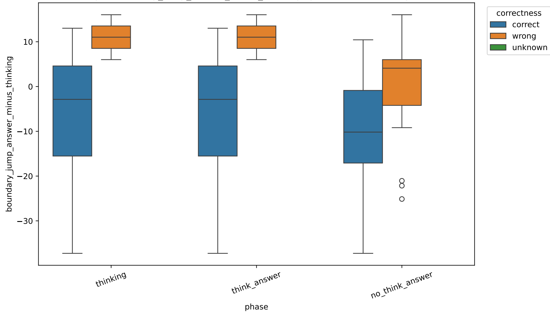
Exp C boundary_jump_answer_minus_thinking by correctness, 4B, layer 6
