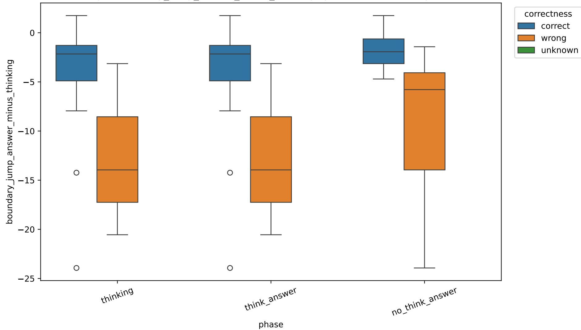
Exp C boundary_jump_answer_minus_thinking by correctness, 8B, layer 20
