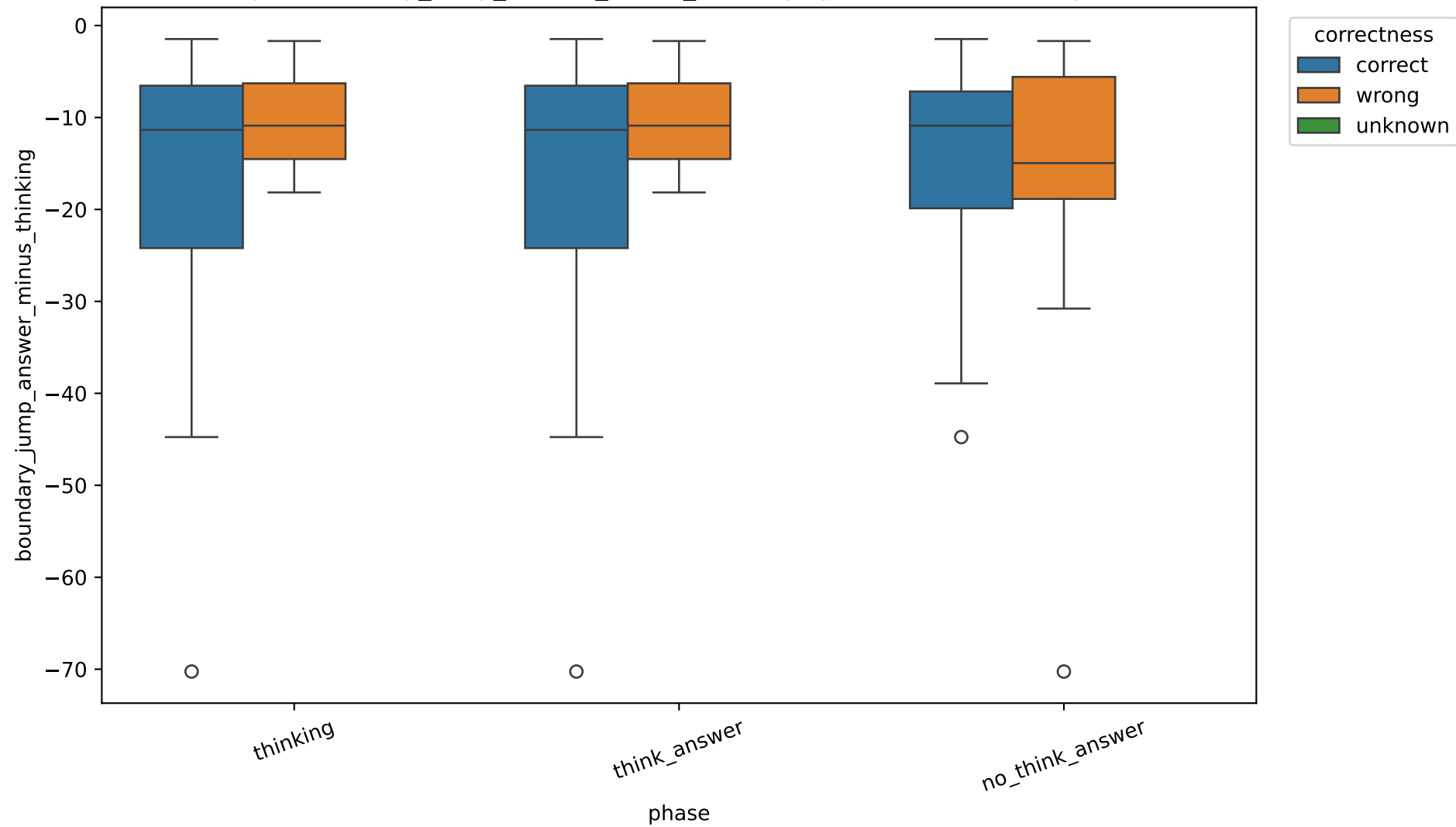
Exp C boundary_jump_answer_minus_thinking by correctness, 8B, layer 6
