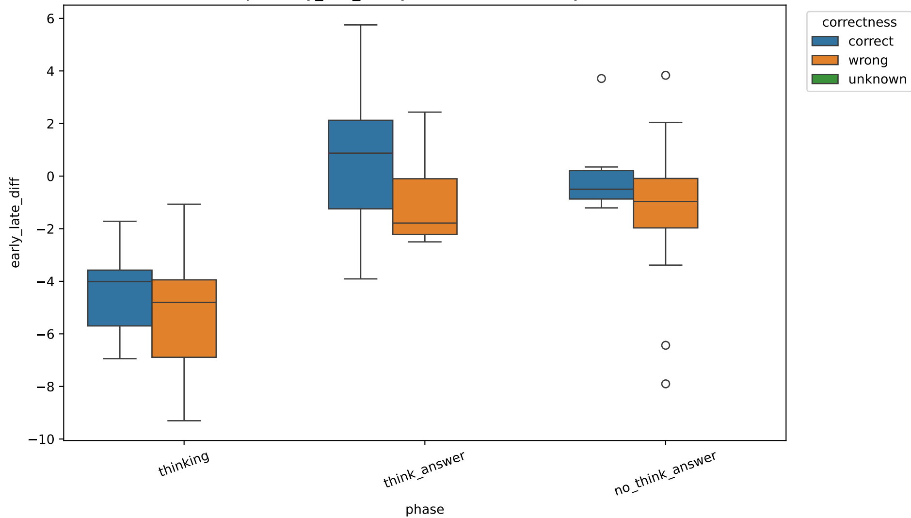
Exp C early_late_diff by correctness, 1.7B, layer 13
