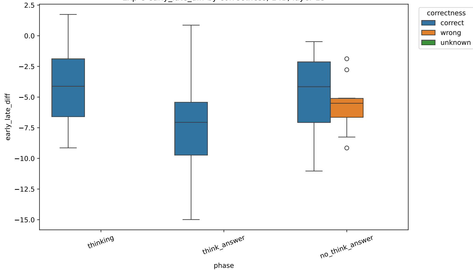
Exp C early_late_diff by correctness, 14B, layer 13
