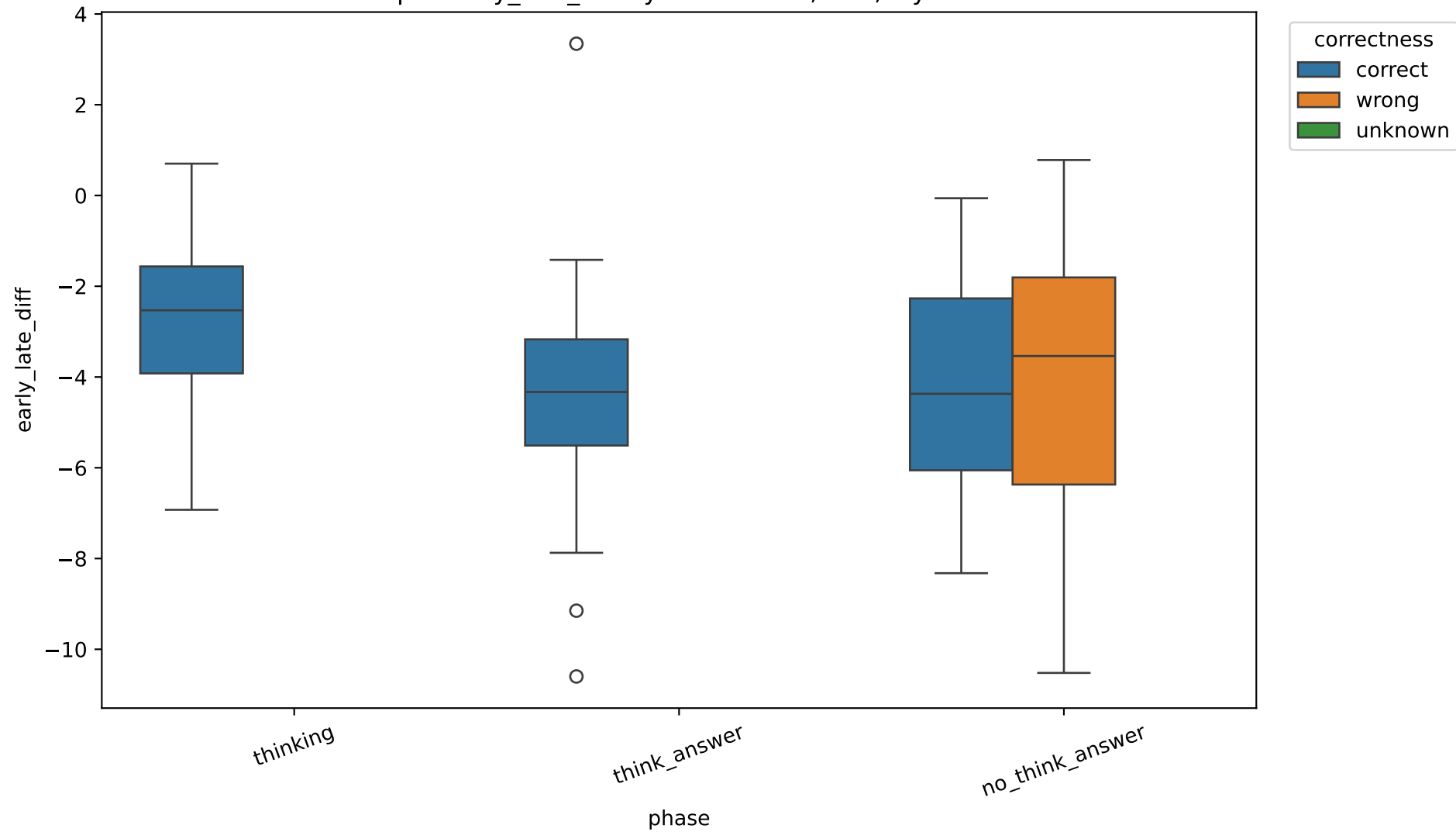
Exp C early_late_diff by correctness, 14B, layer 20
