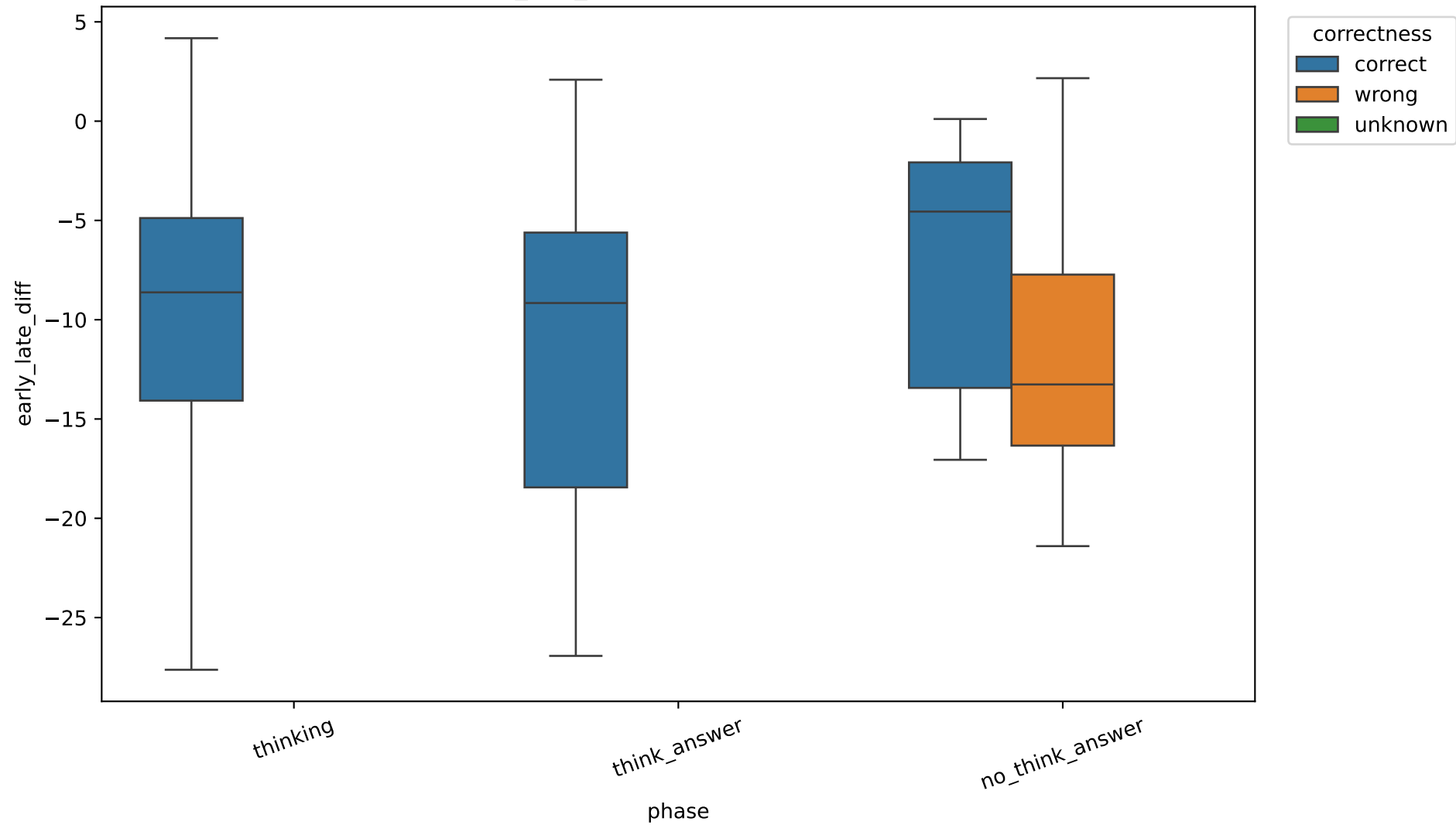
Exp C early_late_diff by correctness, 14B, layer 6
