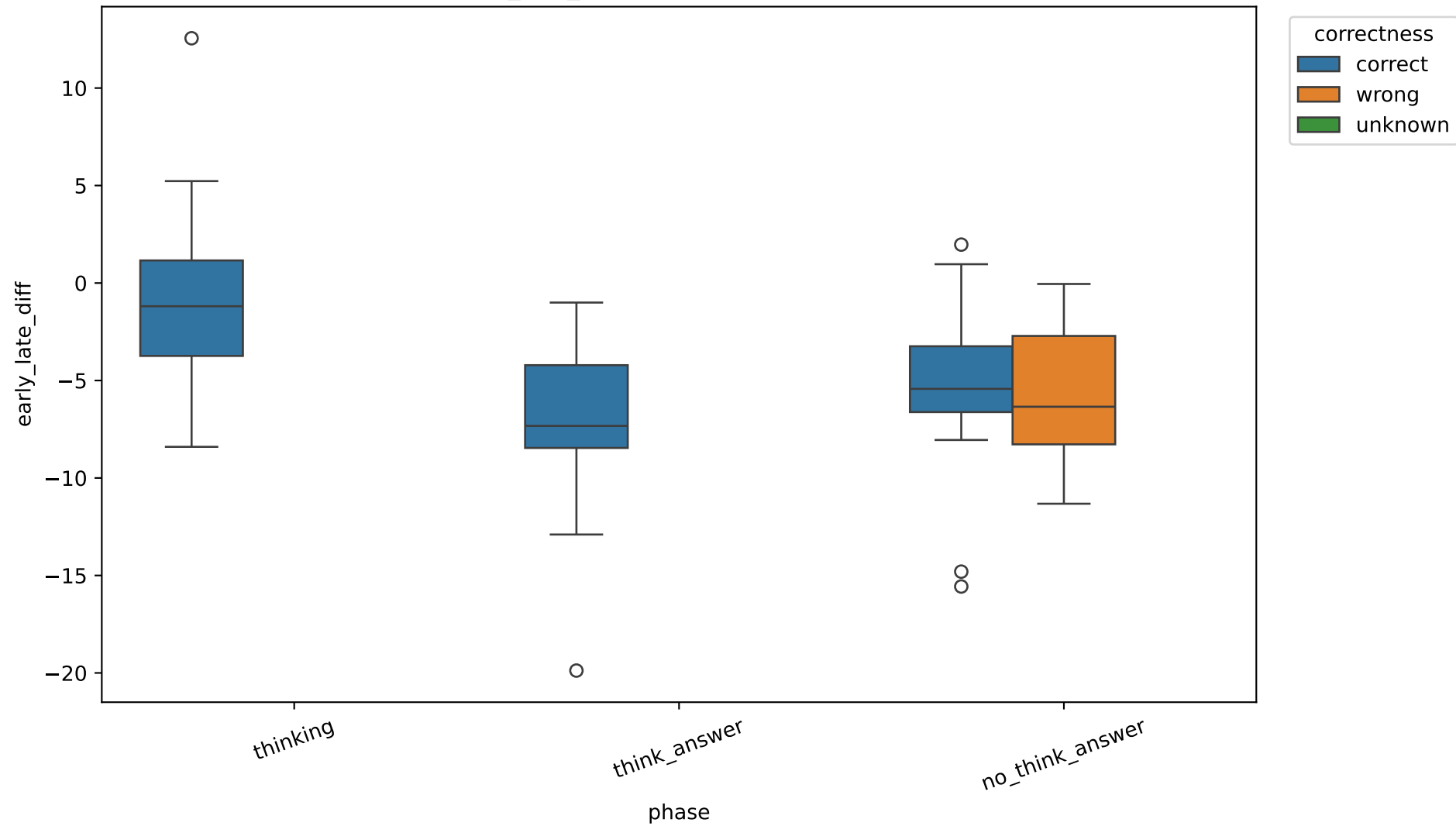
Exp C early_late_diff by correctness, 32B, layer 13
