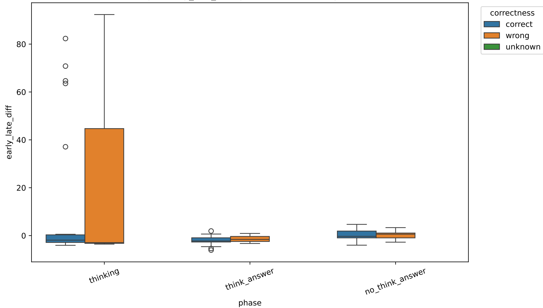
Exp C early_late_diff by correctness, 8B, layer 20
