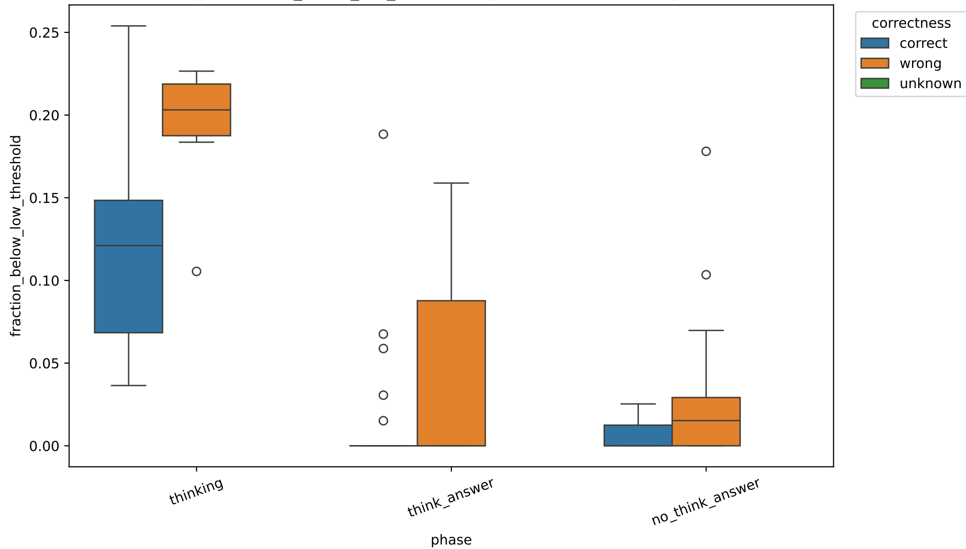
Exp C fraction_below_low_threshold by correctness, 1.7B, layer 13
