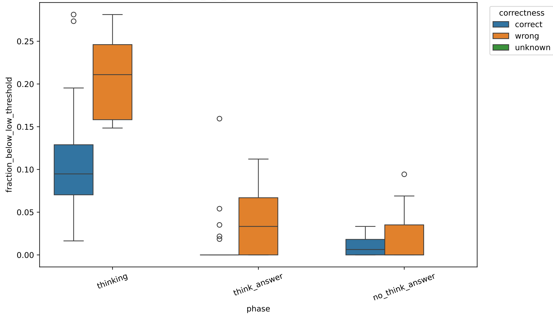
Exp C fraction_below_low_threshold by correctness, 1.7B, layer 20
