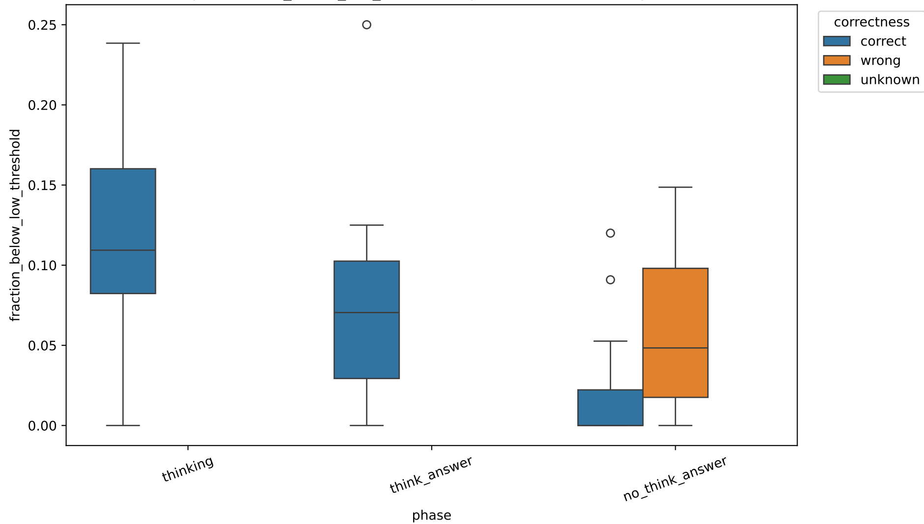
Exp C fraction_below_low_threshold by correctness, 14B, layer 13
