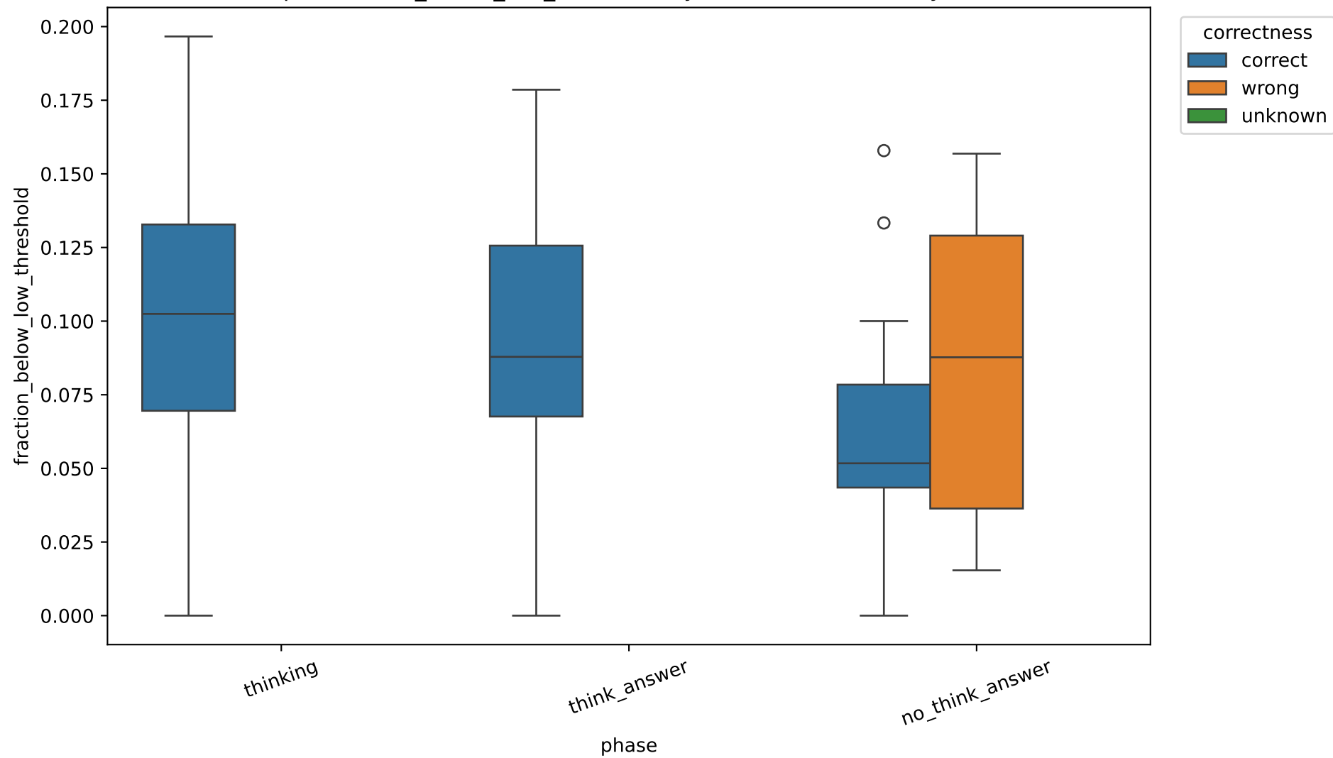
Exp C fraction_below_low_threshold by correctness, 14B, layer 20
