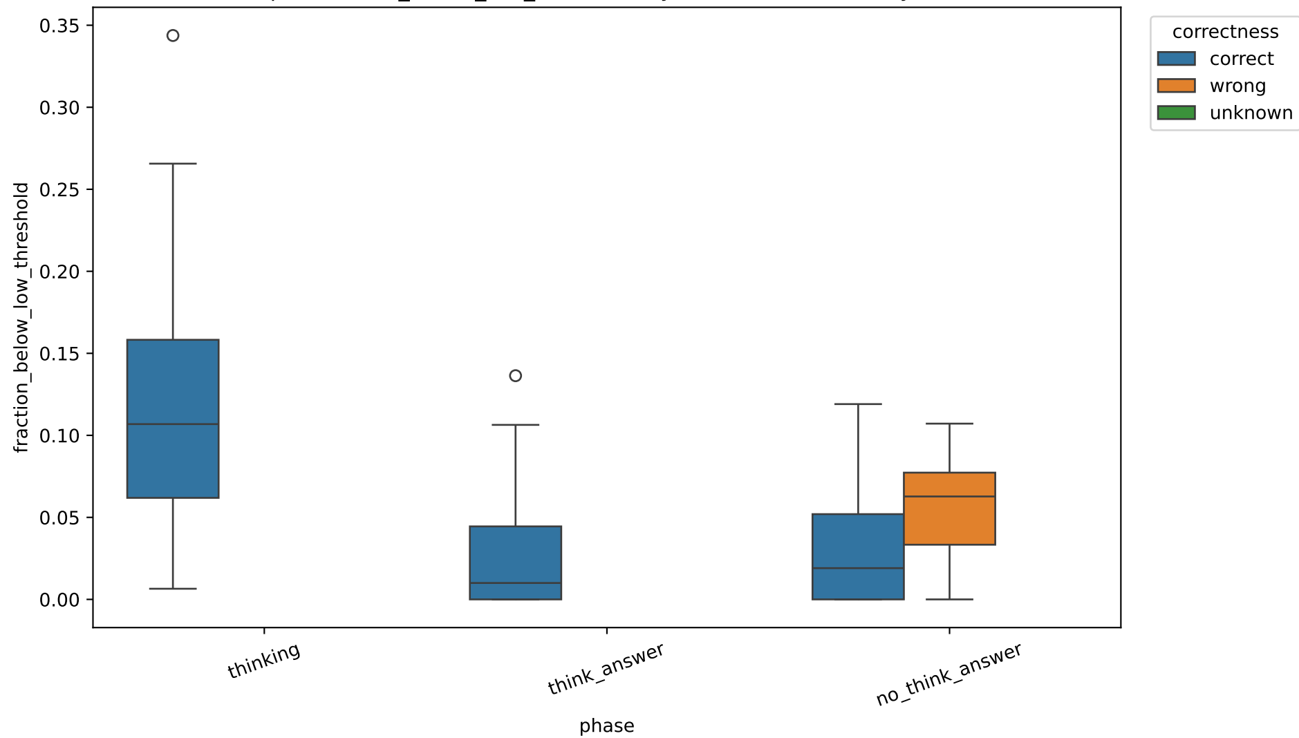
Exp C fraction_below_low_threshold by correctness, 32B, layer 13
