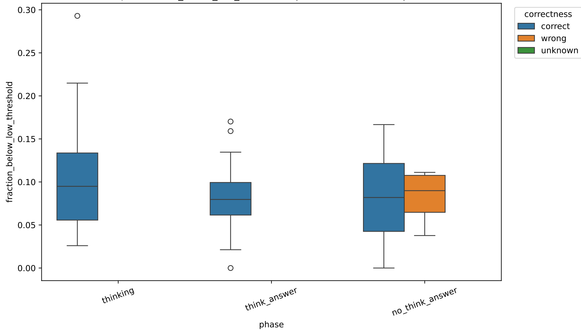
Exp C fraction_below_low_threshold by correctness, 32B, layer 20
