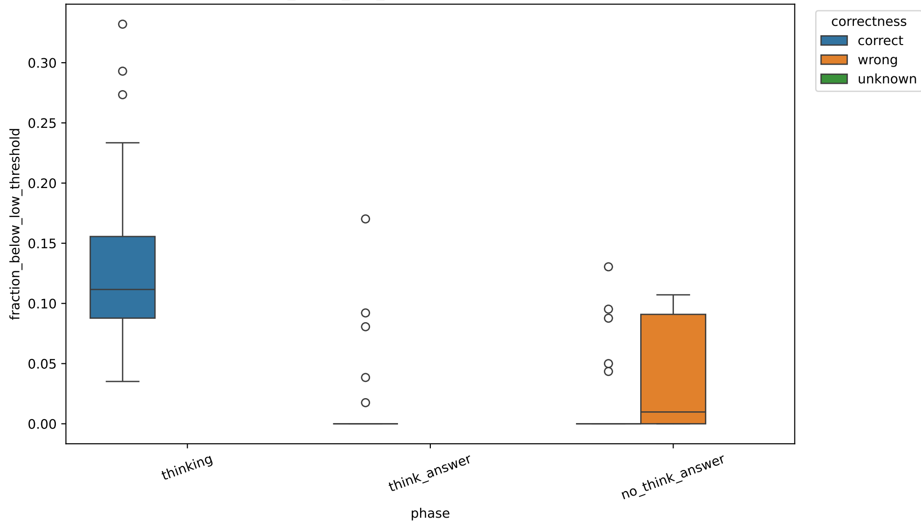
Exp C fraction_below_low_threshold by correctness, 32B, layer 6
