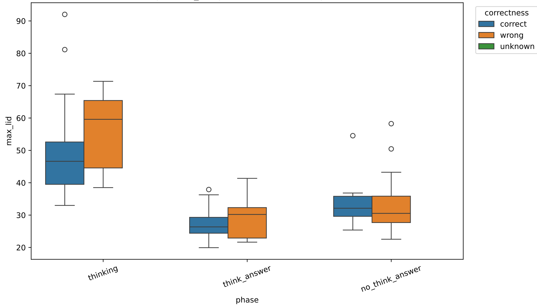
Exp C max_lid by correctness, 1.7B, layer 20
